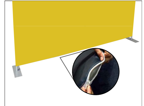
6. Zip up the bottom of the graphic.
